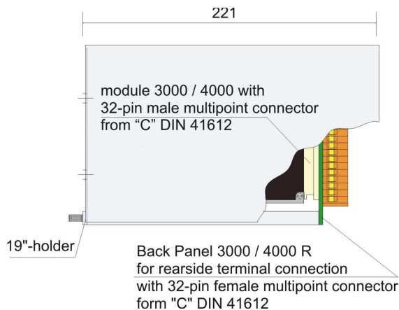
Back Panel 3000 / 4000 R
